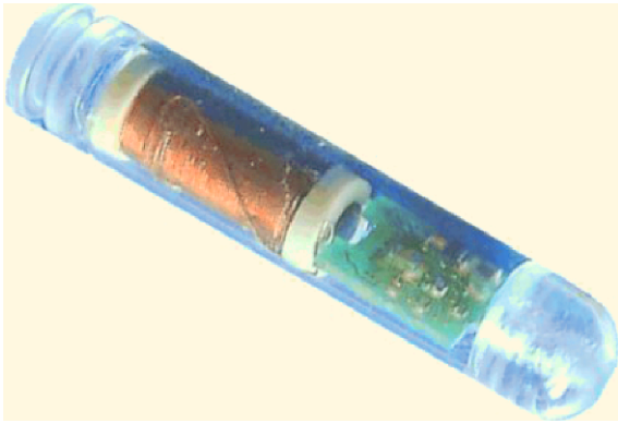
Fig. 11.9 Concept of an implantable blood pressure measurement. Source: Sensorcor, Ltd., Karlsruhe, Germany. The implant is an integrated device that comprises several MST components such as pressure sensors and miniaturized telemetry coils
