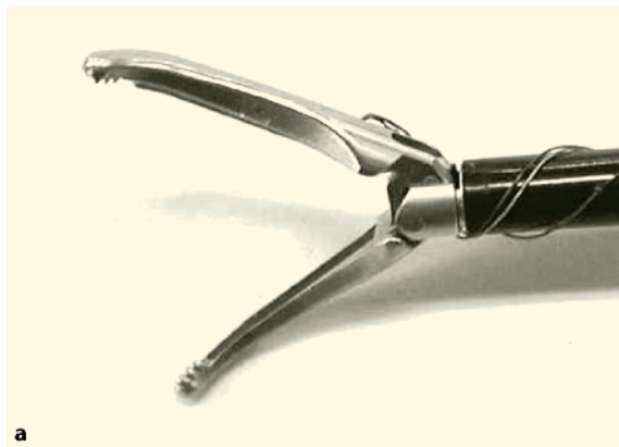
Fig. 13.2 a Closeup of the prototype forceps. The grippers are ideally curved as in the conventional dissecting forceps. b In one of the grippers a heating blade is attached. In the blade a
