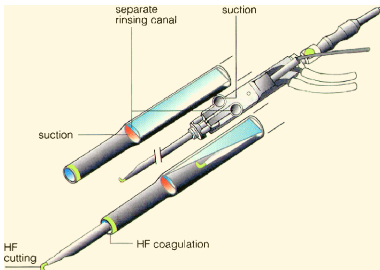
Fig. 12.13 A graphical demonstration of the Wolf combination instruments. Rinsing, suction, and coagulation by the tip are possible by the outer sheath of the combination instrument. The integrated hook allows sharp dissection. The tip can be pulled backward into the shaft of the combination instrument for unrestricted rinsing, suction, and coagulation
